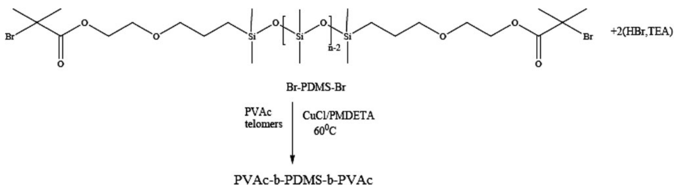
Scheme 3 ATRP route of PVAc telomers initiated with PDMS macroinitiators
