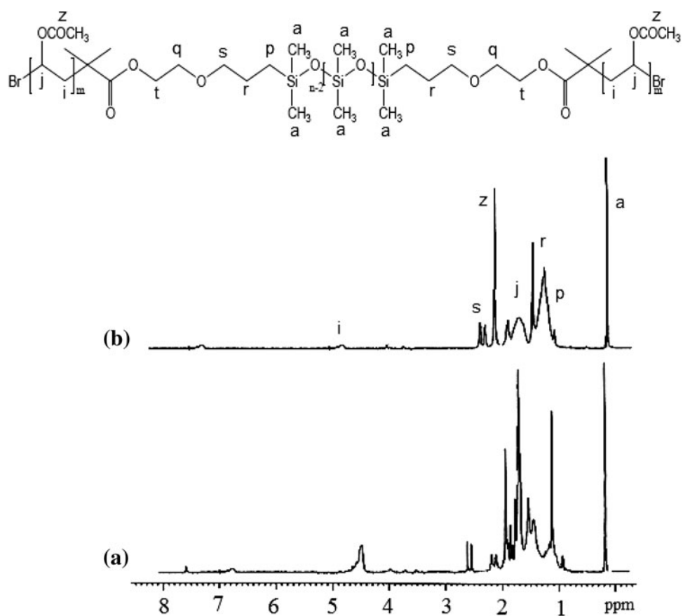
Fig. 5 ^1\text{H} NMR spectrum for the ATRP of PDMS macroinitiator with PVAc telomers from a free radical telomerization, b controlled radical telomerization at 60 °C for 6 h
