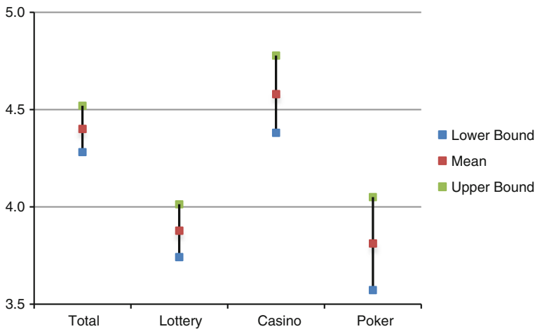
Fig. 1 Mean number of limit events per game type
