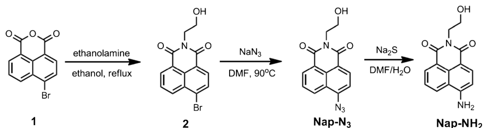
Scheme 2 Synthesis of H 2 S sensor Nap-N 3 and the reduced product Nap-NH 2
