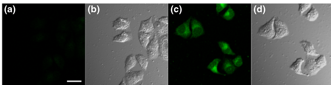
Fig. 8 Confocal fluorescence images of HeLa cells incubated with 5 \mu\text{M} Nap- \text{N}_3 for 20 min ( a, b ) and then 20 \mu\text{M} \text{Na}_2\text{S} for 20 min ( c, d ). Images ( a, c ) were acquired using 405 nm excitation and green emission channels of 520–570 nm; ( b, d ) bright field images. Scale bar = 40 \mu\text{m}
