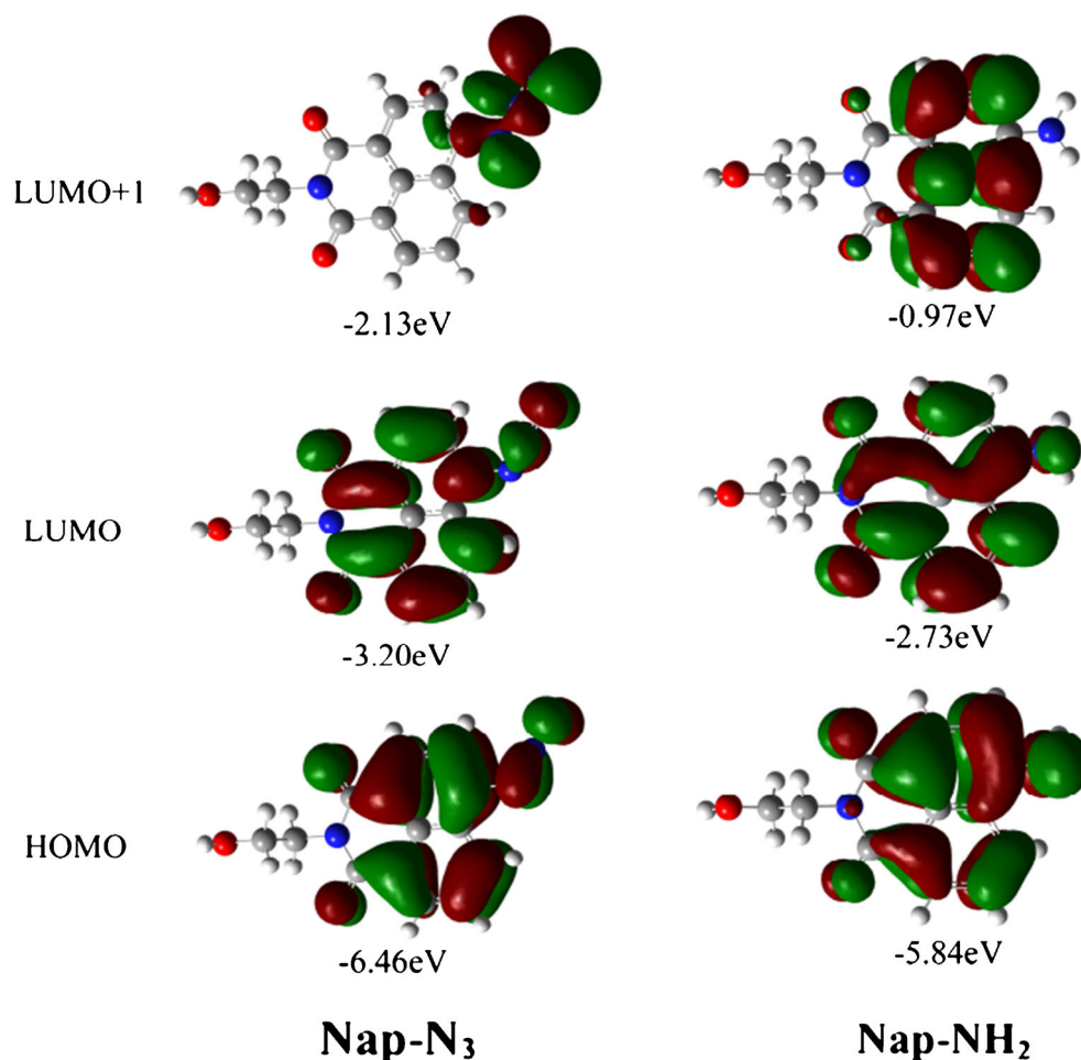
Fig. 4 Interfacial plots of the orbitals for Nap- \text{N}_3 (left) and Nap- \text{NH}_2 (right) in the excited states
