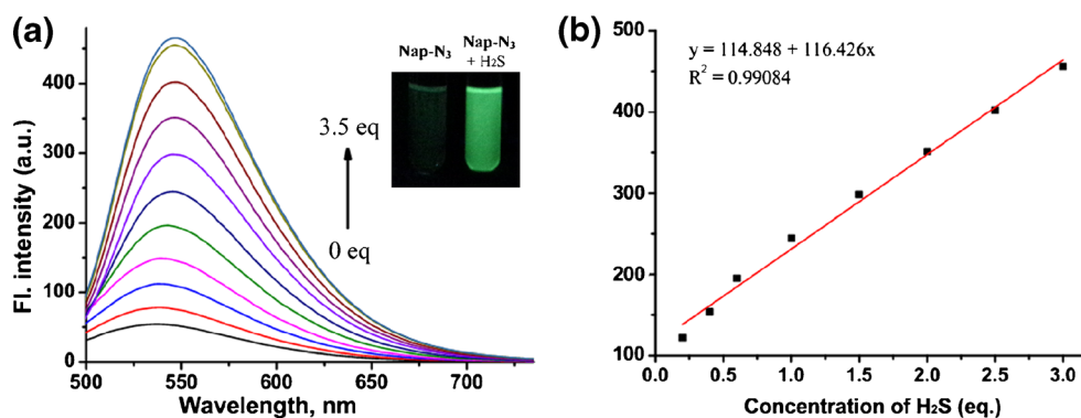
Fig. 1 a Fluorescence spectra ( \lambda_{\text{ex}} = 408 nm) of 10 \mu\text{M} Nap- \text{N}_3 with 0–3.5 eq. of \text{Na}_2\text{S} in 25 mM phosphate buffer (pH 7.4, containing 2 % ethanol). The inset shows the visual fluorescence color of Nap- \text{N}_3
