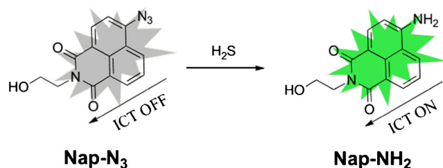
Scheme 1 A turn-on fluorescent H 2 S probe based on the proposed ICT switching mechanism
