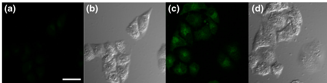
Fig. 9 Confocal fluorescence images of HeLa cells incubated with 5 \mu\text{M} Nap- \text{N}_3 only for 20 min ( a, b ) and 200 \mu\text{M} cysteine for 1 h followed by 5 \mu\text{M} Nap- \text{N}_3 for 20 min ( c, d ). Images ( a, c ) were acquired using 405 nm
