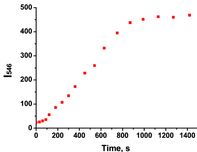
Fig. 6 Time-dependent fluorescence intensity (at 546 nm) responses of sensor Nap-N 3 (10 \mu M) to 3 eq. Na 2 S in PBS buffer
