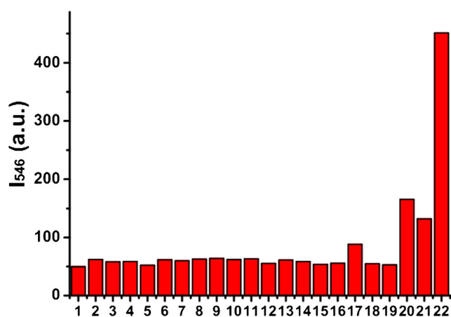
Fig. 5 Fluorescence intensity (at 546 nm) of sensor Nap-N 3 (10 \mu M) in the presence of various analytes in aqueous solution (pH 7.4 PBS, containing 2 % ethanol): 1, blank; 2, F - ; 3, Cl - ; 4, I - ; 5, N 3 - ; 6, CO 3 2- ; 7, SO 4 2- ; 8, HPO 4 2- ; 9, NO 2 - ; 10, NO 3 - ; 11, Ac - ; 12, SCN - ; 13, citrate; 14, S 2 SO 3 2- ; 15, ClO - ; 16, H 2 O 2 ; 17, SO 3 2- ; 18, NO; 19, ascorbic acid; 20, Cys; 21, GSH; 22, Na 2 S
