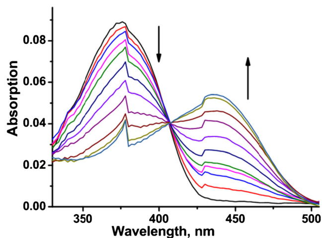
Fig. 2 Absorption spectra of probe Nap- \text{N}_3 with 0–3.5 eq. of \text{Na}_2\text{S} in 25 mM phosphate buffer (pH 7.4, containing 2 % ethanol)
