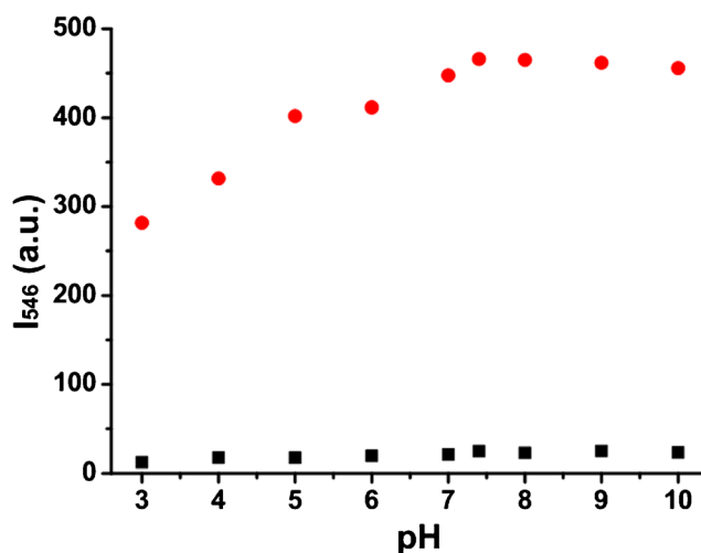
Fig. 7 The pH influence on the fluorescence intensity (at 546 nm) of Nap-N 3 (10 \mu M) in the absence (black square) or presence (red circle) of Na 2 S (30 \mu M)
