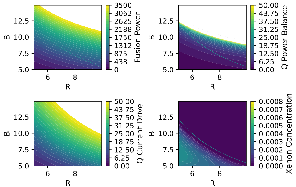
Fig. 3 Contours of P_{fus} , Q_{PB} , Q_{CD} and f_{Xe} in the R, B plane for the ASDEX Upgrade hybrid scenario. The green line is the synchrotron limit, f_{sync} = 1 (Color figure online)
