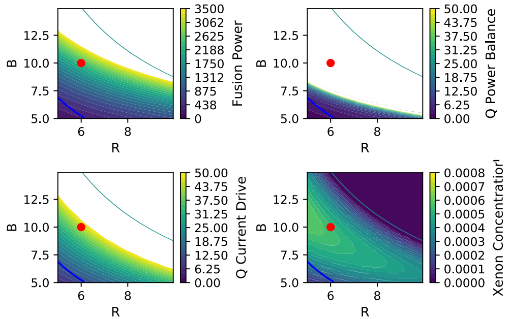
Fig. 5 Contours of P_{fus} , Q_{PB} , Q_{CD} and f_{Xe} in the R, B plane for the DIII-D/EAST scenario. The red point represents an examples at (6 m, 10 T) discussed in the text, the blue line indicates the exhaust similarity scaling to the ITER Q = 10 scenario. The green line is the synchrotron limit f_{sync} = 1.0 (Color figure online)
