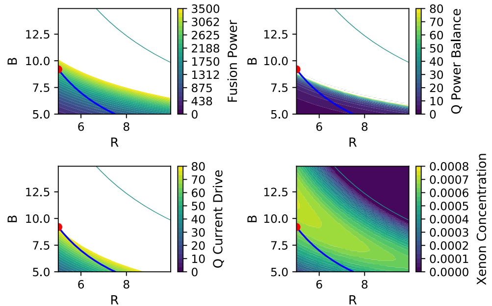
Fig. 6 Contours of P_{fus} , Q_{PB} , Q_{CD} and f_{Xe} in the R, B plane for an scenario optimized for compact steady state tokamak operation at low recirculating power. The red point represents an example at (5 m, 9.3 T) discussed in the text, the blue line indicates the exhaust similarity scaling to the ITER Q = 10 scenario. The green line is the synchrotron limit f_{sync} = 1.0 (Color figure online)
