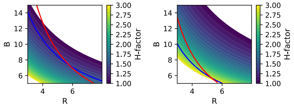
Fig. 7 Left: contours of the H-factor needed for Q_{PB} = 80 for the parameter set from Fig. 6 ( \beta_N = 4.0 , f_{GW} = 1.2 , q_{95} = 5.7 ). The red line shows the ITER exhaust similarity line, the blue line the line on which Q_{CD} = 80 . Right: the same for a more conservative set ( \beta_N = 3.0 , f_{GW} = 1.0 , q_{95} = 8.3 ) (Color figure online)
