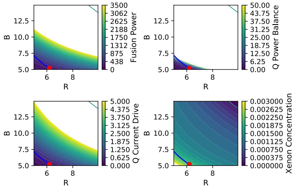
Fig. 2 Contours of P_{fus} , Q_{PB} , Q_{CD} and f_{Xe} in the R, B plane for the ITER Q = 10 scenario. The red dot represents the ITER Q = 10 operational point, the blue line indicates the exhaust similarity scaling, the green line is the synchrotron limit, in this case taken to be f_{sync} = 0.8 . Note that the scale for Q_{CD} is a factor of 10 lower than for the following plots, and the scale for f_{Xe} is higher by a factor of 3.75 (Color figure online)
