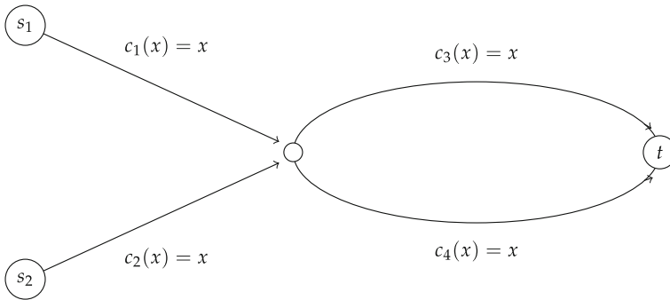
Fig. 1 Multiple equilibria
