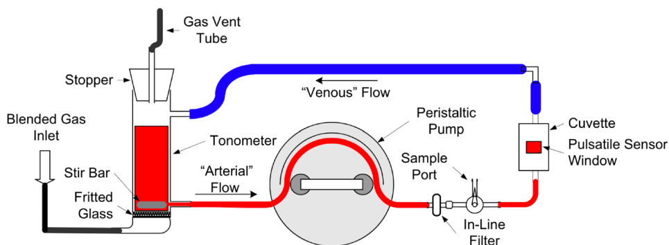
Fig. 1 Simplified schematic of in vitro circulation system [16]
