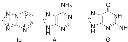
Scheme 1 The ligand [1,2,4]triazolo[1,5-a]pyrimidine (tp) and its IUPAC recommended ring-atom numbering system, together with adenine (A) and guanine (G)
