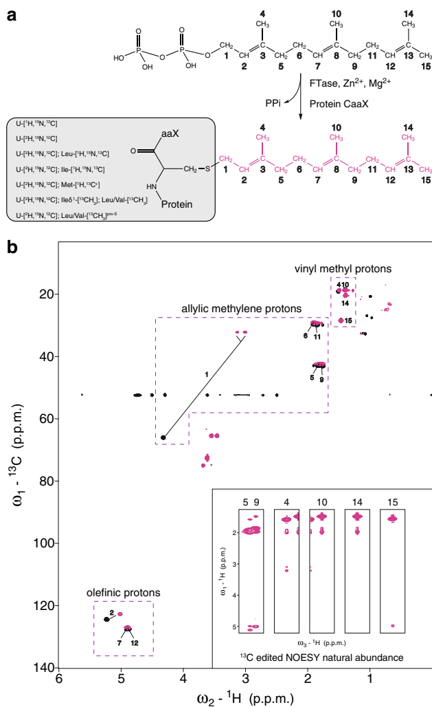
Fig. 2 Sampling the farnesyl resonances. a Schematic representation of in vitro farnesylation reaction for any target protein containing the CaaX box. Farnesyl groups are numbered. Any labeling scheme, as the ones listed for the present study, can be applied to the protein before the attachment of the unlabeled farnesyl. b Natural abundance ^{13}\text{C}, ^1\text{H} HSQC spectra of farnesylated PEX19 labeled with ^2\text{H} -glucose (magenta) and farnesyl pyrophosphate dissolved in methanol (black). In either case, farnesyl resonances are numbered as shown in a . Inset shows NOE strips from a natural abundance ^{13}\text{C} -edited 3D NOESY spectrum recorded on perdeuterated PEX19 using non-uniform sampling. Numbers at the top indicate the edited farnesyl resonances
