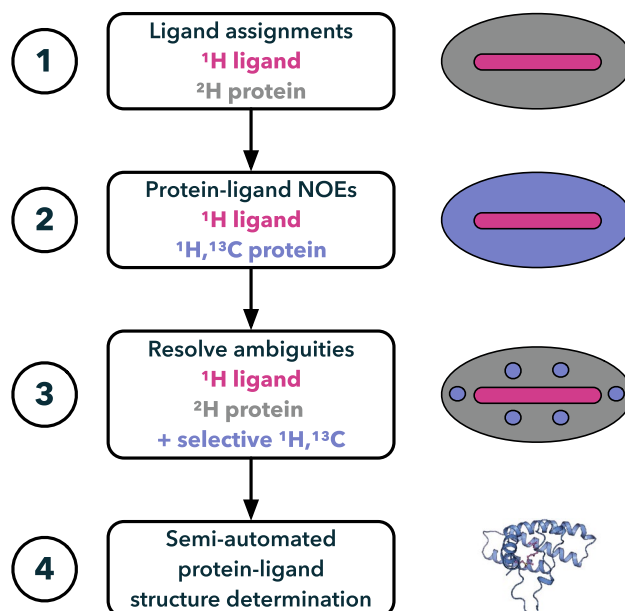
Fig. 1 Flowchart and NMR labeling schemes that allow identifying ligand frequencies (1), collecting protein–ligand NOEs (2), and resolving NOE ambiguities (3) for structure determination of protein–ligand complexes (4)
