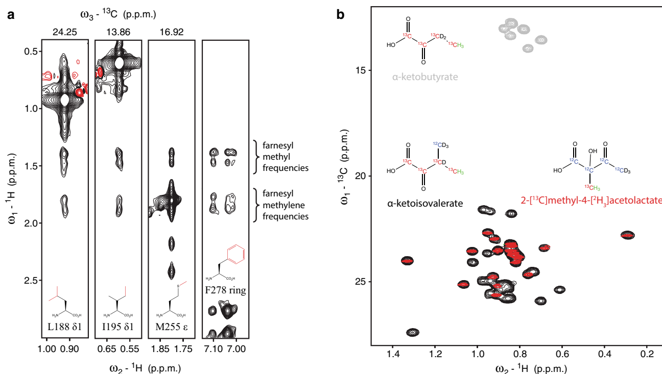
Fig. 4 Labeling schemes for mapping protein-farnesyl contacts. a Strips from {}^{13}\text{C} -edited NOESY spectra recorded on samples specifically labeled for the methyl groups of leucine, isoleucine, and methionine (highlighted in red in the schematic representation of amino acids) and the aromatic portion of a 2D homonuclear NOESY spec-
