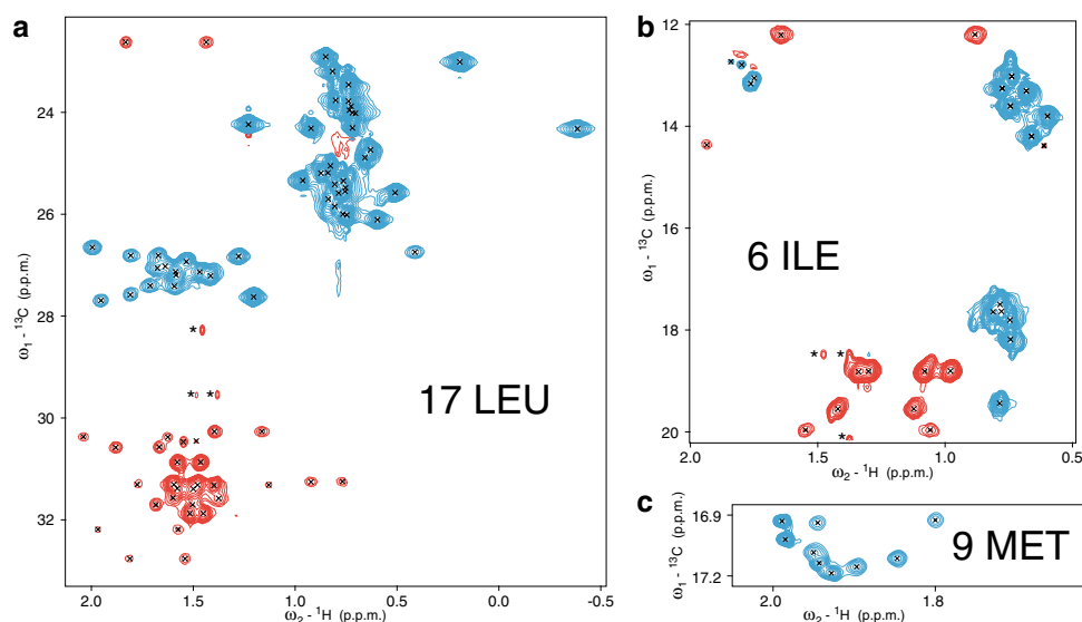
Fig. 3 NMR spectra recorded for amino acid selectively-labeled, perdeuterated and uniformly ^{15}\text{N} -labeled PEX19 protein with unlabeled farnesyl covalently attached. a Constant time ^{13}\text{C}, ^1\text{H} HSQC spectrum of perdeuterated PEX19 expressed with ^1\text{H}/^{15}\text{N}/^{13}\text{C} leucine. b Constant time ^{13}\text{C}, ^1\text{H} HSQC spectrum of perdeuterated PEX19 expressed with ^1\text{H}/^{15}\text{N}/^{13}\text{C} isoleucine. c ^{13}\text{C}, ^1\text{H} HSQC spectrum of perdeuterated PEX19 expressed with ^1\text{H}/^{13}\text{C} methionine. In all cases the \alpha proton of the amino acid precursor has been replaced by a deuteron of the solvent. All ^1\text{H}-^{13}\text{C} resonance pairs are observed. Positive peaks are coloured cyan and negative peaks are coloured red. Asterisks indicate natural abundance methyl crosspeaks of the attached farnesyl
