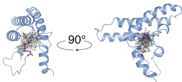
Fig. 5 Two views of the solution NMR structure of farnesylated PEX19 (PDB:5LNF). Each black line corresponds to an NOE distance restraint between the protein and the farnesyl moiety. The distance network comprises 203 NOEs recorded on samples using various labeling schemes
