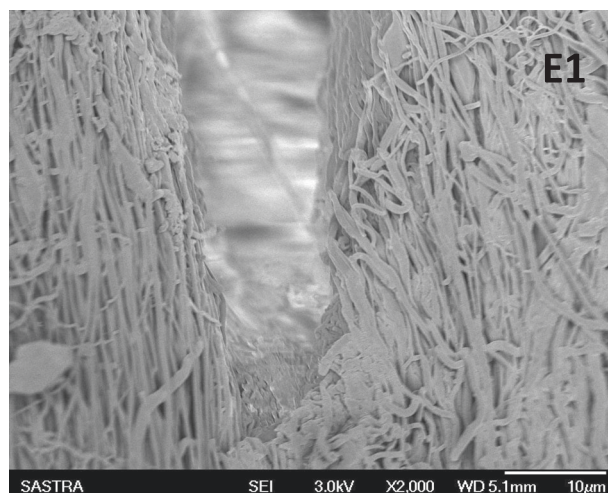
Fig. 2 Scanning electron micrograph showing the orientation of fiber angle of PLGA–PHT nanofiber at rotation speed: 2,000 rpm
