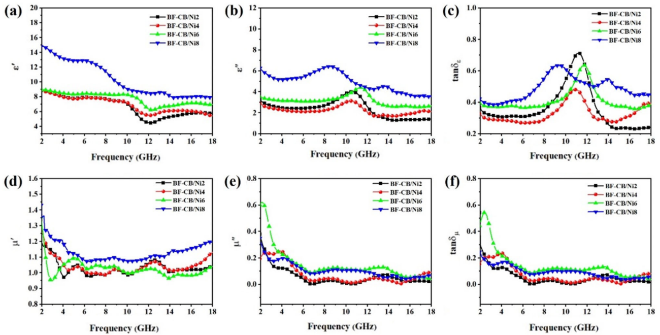
Fig. 7 Frequency dependence of complex permittivity (a, b), dielectric loss tangent (c), complex permeability (d, e) and magnetic loss tangent (f) of BF-CB/Ni 2 , BF-CB/Ni 4 , BF-CB/Ni 6 , BF-CB/Ni 8
