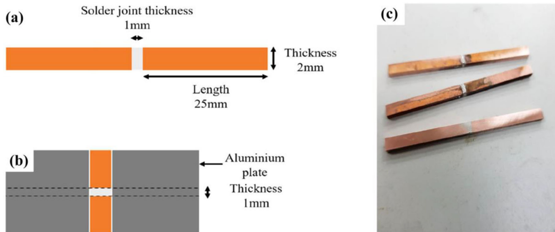
Fig. 1 Experimental procedure for the preparation of Sn-58Bi- x Co tensile samples
