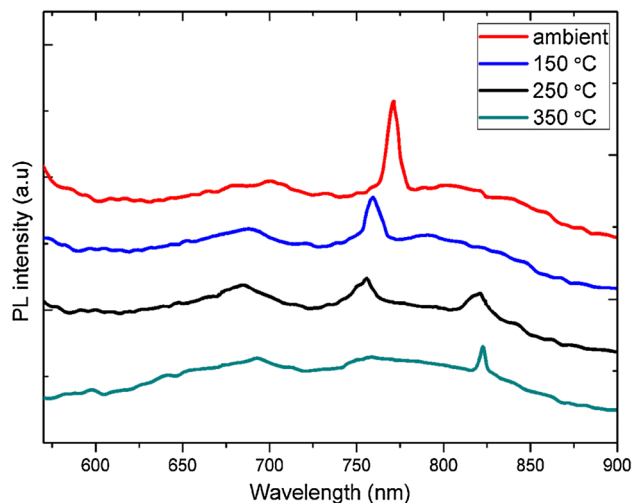
Fig. 8 PL spectra of PbTe–InSe multilayer nanocomposite excited at 500 nm at room temperature
