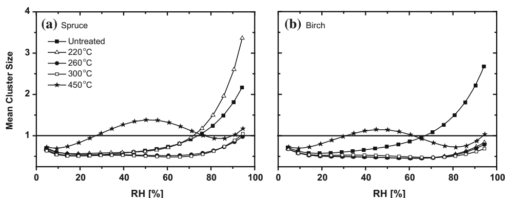
Fig. 4 Clustering of sorbed water molecules in birch and spruce determined using the Zimm–Lundberg approach
