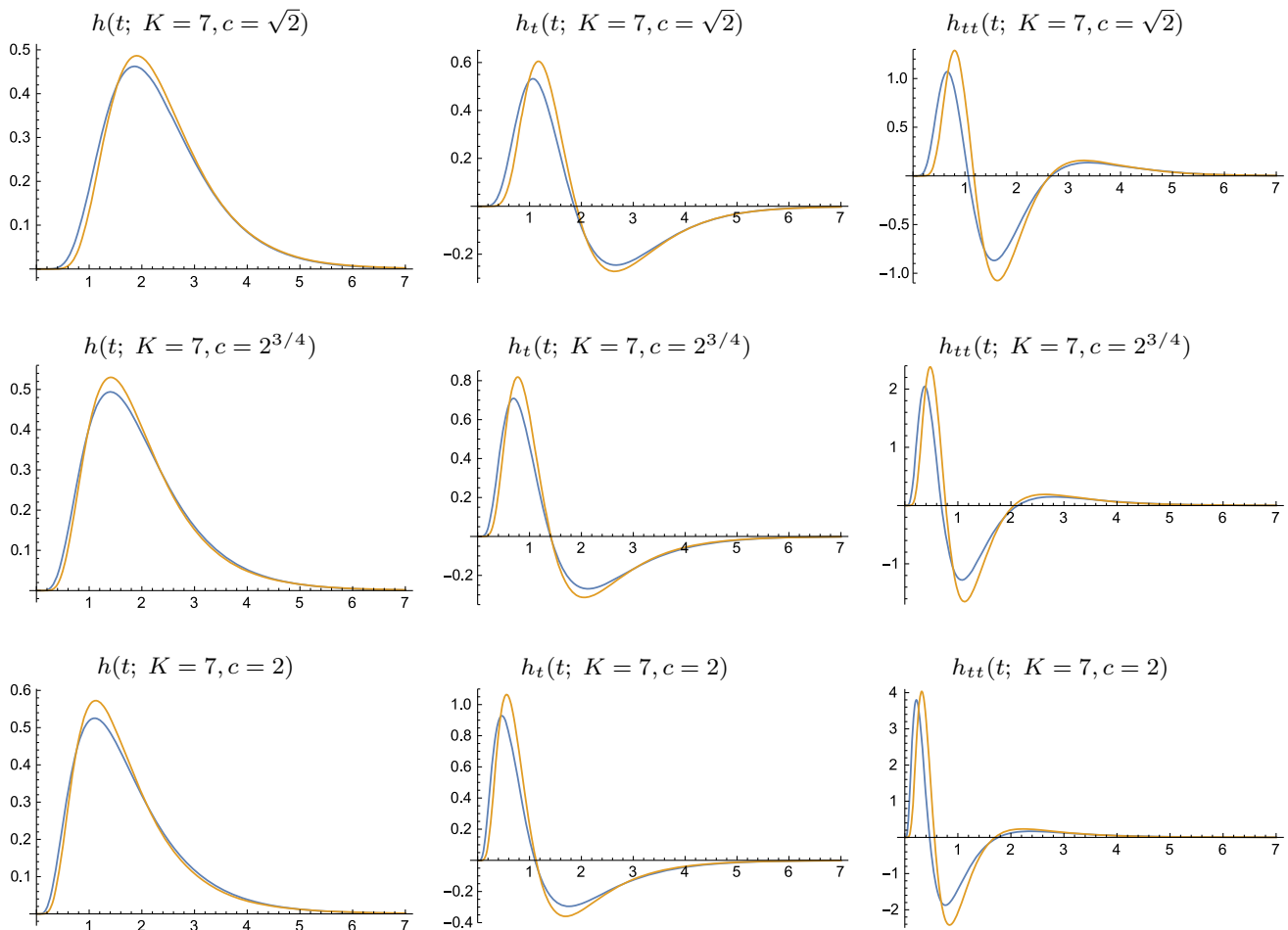
Fig. 11 Comparison between the proposed time-causal kernels corresponding to the composition of truncated exponential kernels in cascade (blue curves) for a logarithmic distribution of the intermediate scale levels and the temporal kernels in Koenderink’s scale-time model (brown curves) shown for both the original smoothing kernels and their first and second-order temporal derivatives. All kernels correspond to temporal scale (variance) \tau = 1 with the additional parameters determined
