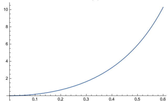
Fig. 10 Graphs of the skewness measure \gamma_1 (157) and the kurtosis measure \gamma_2 (158) as function of the dimensionless temporal scale parameter \sigma relative to the logarithmic transformation of the past for the time-causal kernels in Koenderink’s scale-time model
