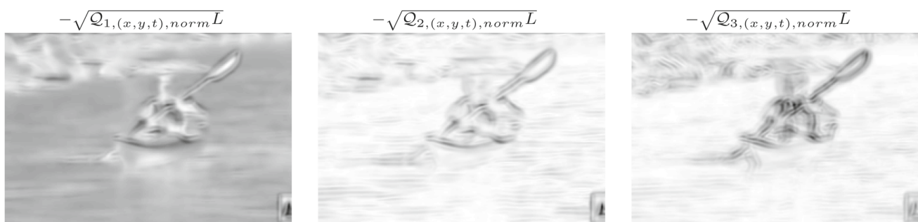
Fig. 8 Illustration of the influence of temporal illumination or exposure compensation mechanisms on spatio-temporal receptive field responses, computed from the video sequence Kayaking_g01_c01.avi (cropped) in the UCF-101 dataset. Each figure shows a snapshot at frame 8 for the quasi quadrature entity shown above the figure with additional monotone stretching of the magnitude values to simplify visual interpretation. Note how the time-varying illumination or exposure
