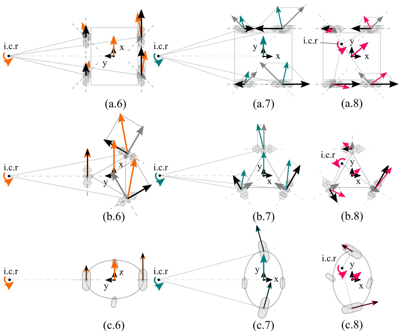
Fig. 10 Velocity analysis of the three architectures (4WD (a.i), 3WD (b.i) and (2SWD(c.i)) during three acts of motion: \dot{X}_b/\dot{\Gamma}_b = 4 (x.6), \dot{Y}_b/\dot{\Gamma}_b = 1 (x.7), generic configuration (x.8)
