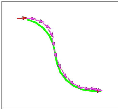
Fig. 2 Example of reference trajectory computed using Dubins curves and connecting two adjacent vertices. The green line is the reference trajectory, whereas magenta arrows are the state trajectory computed using MPC
