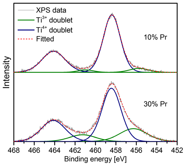
Fig. 6 Ti 2p core-level region for reduced Pr30% and Pr10% samples
