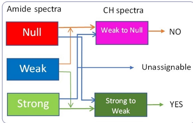
Fig. 18 Problem to solve: “Does the trace contain organic materials?” According to the PCA analysis of the infrared data, there are three pathways to answer the question: green lines yield a favorable answer, the red ones to reject the hypothesis. The blue lines drive toward unclear answer
