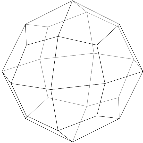
Fig. 2 The rational polytope P = \{x \in \mathbf{R}^3 \mid |x_1| + |x_2| + |x_3| + \max\{|x_1|, |x_2|, |x_3|\} \leq 1\} . Its Ehrhart series can be computed by Corollary 4.6
