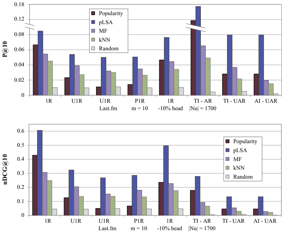
Fig. 8 Precision and nDCG of recommendation algorithms on MovieLens 1M (and Last.fm only where indicated) using the 1R, UIR, P1R ( m = 10 percentiles), AR, and UAR methodologies. The “–10% head” bars show the effect of removing the 10% most popular items from the test data (Cremonesi et al. 2010)
