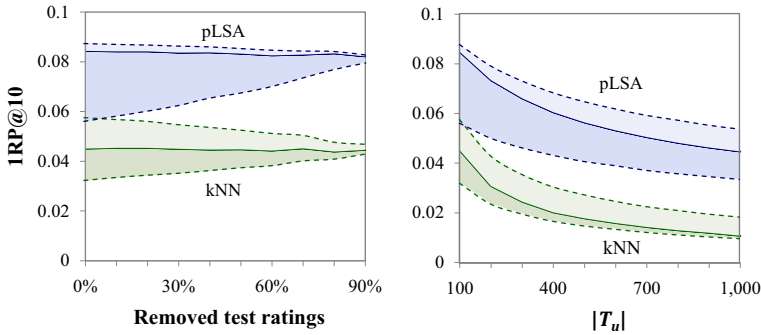
Fig. 3 Empirical illustration of Eq. (2). The curves show IRP@10 and its bounds, for pLSA and kNN over MovieLens 1M. The light and dark shades mark the distance to the upper and lower bounds, respectively. The left side shows the evolution when progressively removing test ratings, and the right side displays the variation with |T_u| ranging from 100 to 1000
