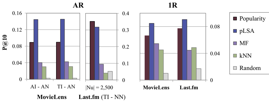
Fig. 2 Precision of different recommendation algorithms on MovieLens 1M and Last.fm using AR and IR configurations
