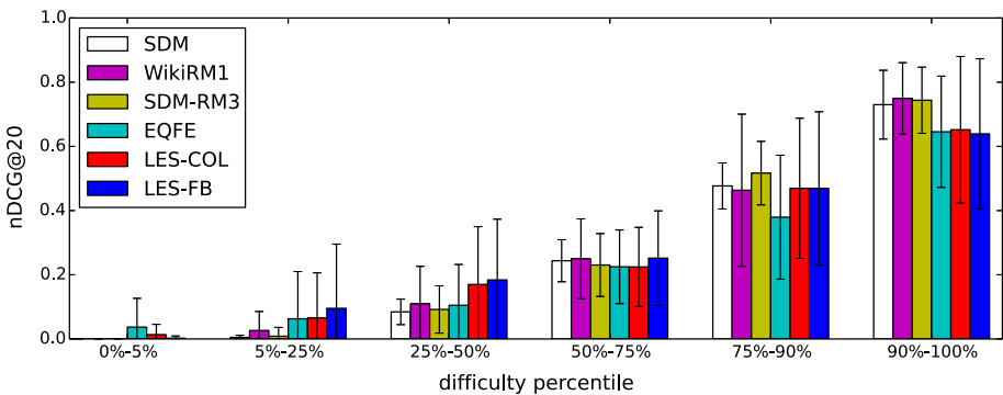
Fig. 8 Mean performance (nDCG@20) of different query difficulties on ClueWeb09 Category B data (TREC 2009–2012). Queries are grouped based on the percentile of SDM. Error bars represent standard deviation
