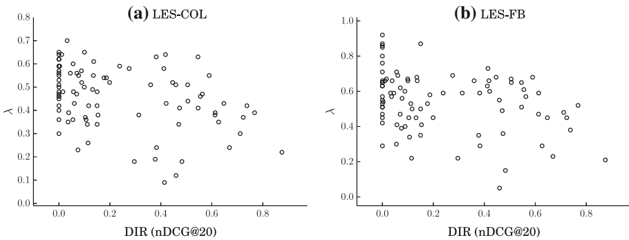
Fig. 5 Correlation between query difficulty (nDCG@20 of DIR) and learned \lambda
