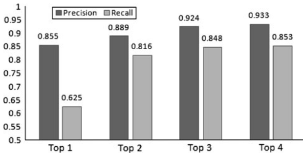
Fig. 5 Precision and recall for the Purdue faculty members with top 1, top 2, top 3 and top 4 returned results, respectively
