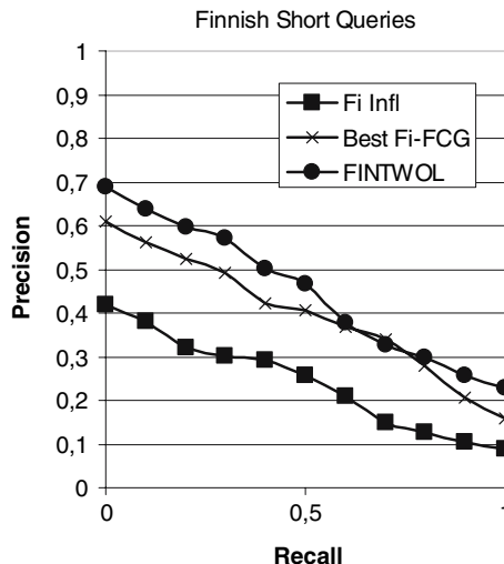
Fig. 9 P/R curves for Finnish short queries: precision by eleven recall levels 0.0–1.0
