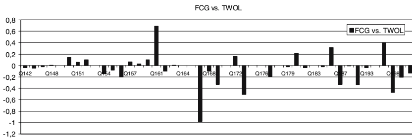
Fig. 1 Query-by-query results of Finnish title-only queries. Best FCG vs. best lemmatization
