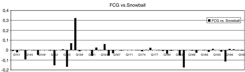
Fig. 5 Query-by-query results of German title-only queries. Best FCG vs. best stemming
