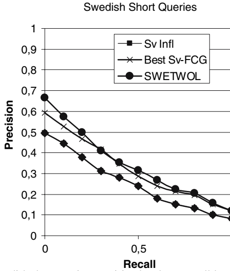
Fig. 10 P/R curves for Swedish short queries: precision by eleven recall levels 0.0–1.0
