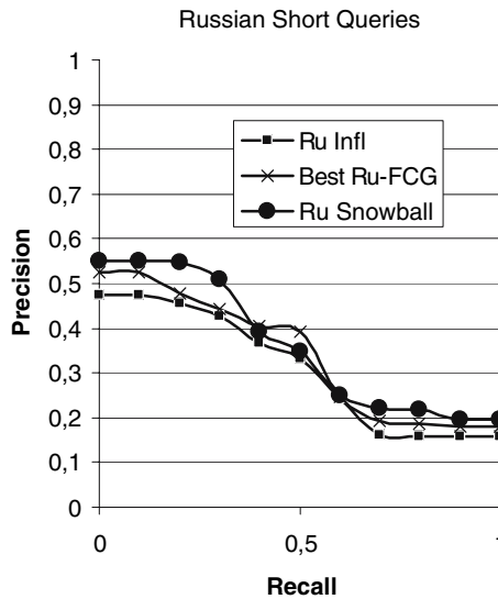
Fig. 12 P/R curves for Russian short queries: precision by eleven recall levels 0.0–1.0
