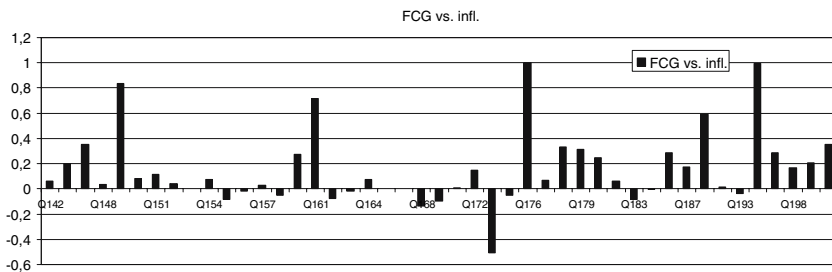
Fig. 2 Query-by-query results of Finnish title-only queries. Best FCG vs. inflected queries
