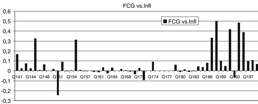
Fig. 4 Query-by-query results of Swedish title-only queries. Best FCG vs. inflected queries
