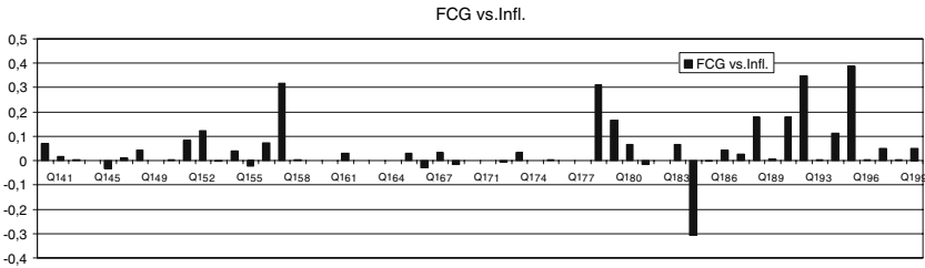
Fig. 6 Query-by-query results of German title-only queries. Best FCG vs. inflected queries
