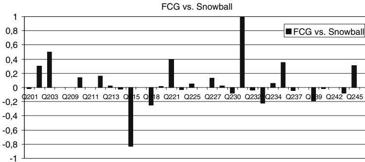
Fig. 7 Query-by-query results of Russian title-only queries. Best FCG vs. stemmed queries
