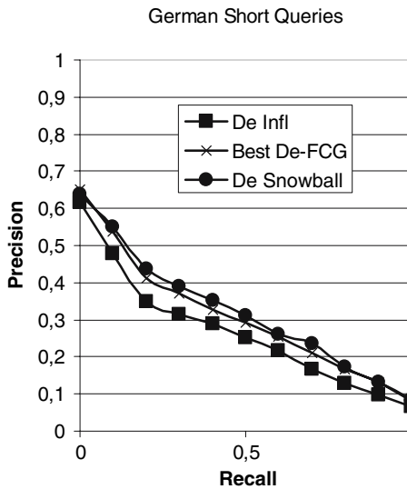
Fig. 11 P/R curves for German short queries: precision by eleven recall levels 0.0–1.0
