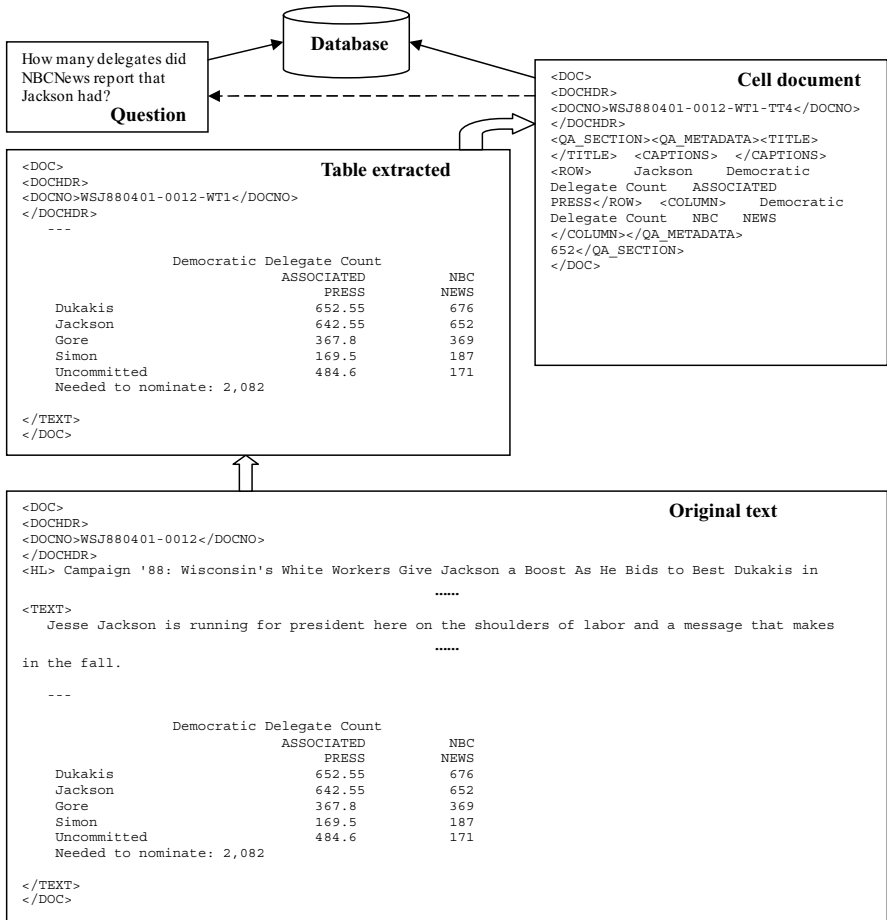
Fig. 6 An example of answer retrieval
