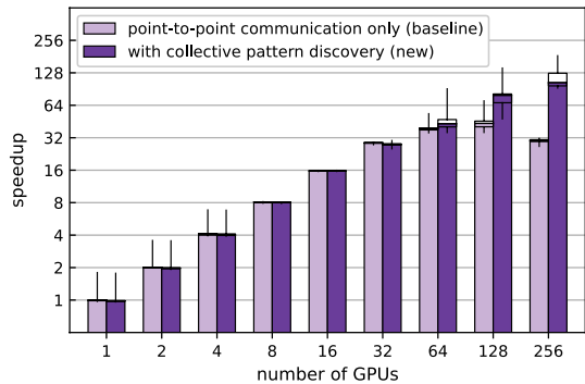
Fig. 4 Throughput of communication-only system benchmarks from Table 3 with kernel execution disabled (higher is better). Shown is a mixed bar-box plot containing the median, center quartiles and minima / maxima over 20 runs on varying node configurations. Each measurement is the mean over 20 iterations
