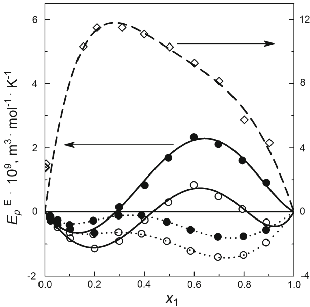
Fig. 3 Excess molar isobaric expansions of the systems: 2,4,6-trimethylpyridine (1) + a proton-donating substance (2). Substance: methanol— dotted lines , 1,2-ethanediol— solid lines , water— dashed line . Points—experimental results: open circles — T = 283.15 K, filled circles — T = 313.15 K, diamonds — T = 277.15 K. Lines—Redlich-Kister polynomials
