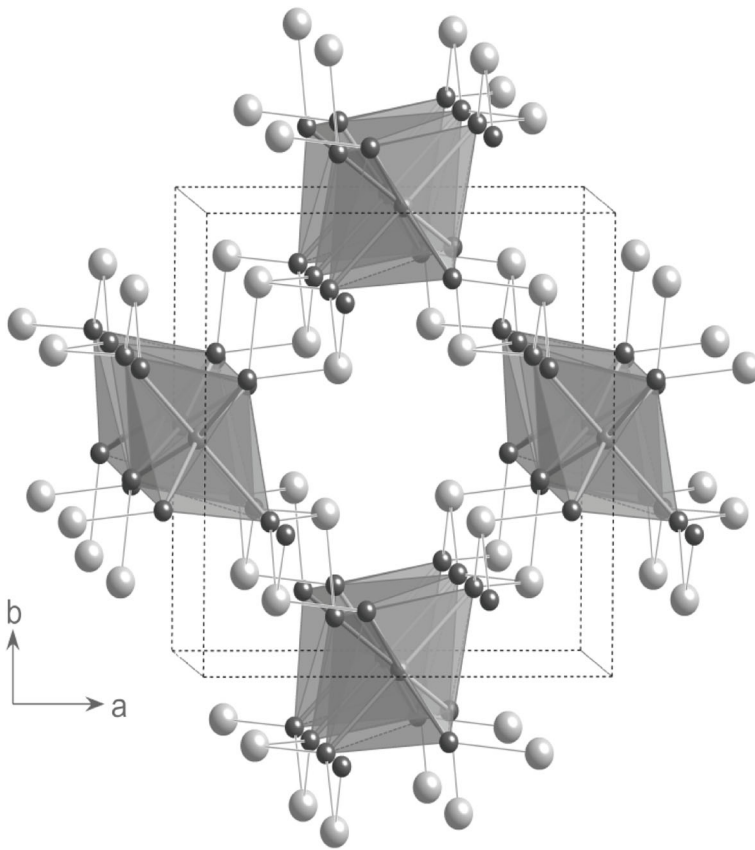
Fig. 1 The structure of FeSb 2 O 4 : FeO 6 octahedra are shaded with Fe 2+ ions located within the octahedra; O 2- ions are shown as black spheres and Sb 3+ ions are shown as white spheres
