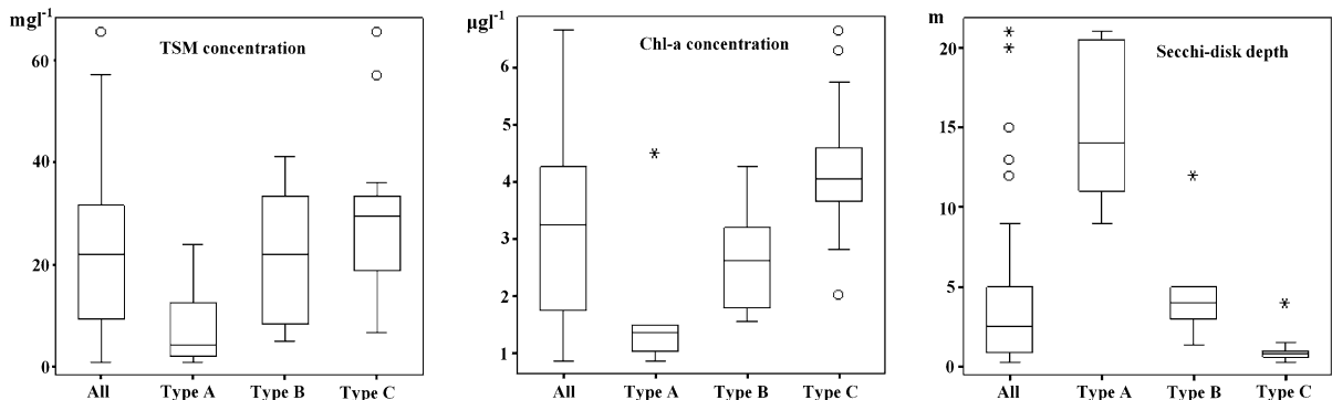
Fig. 2 Box plot of the TSM, Chl a , and Secchi disc depth for all in situ data plotted per water types A, B and C. Boxes indicate the variations as defined by the standard deviation; the
