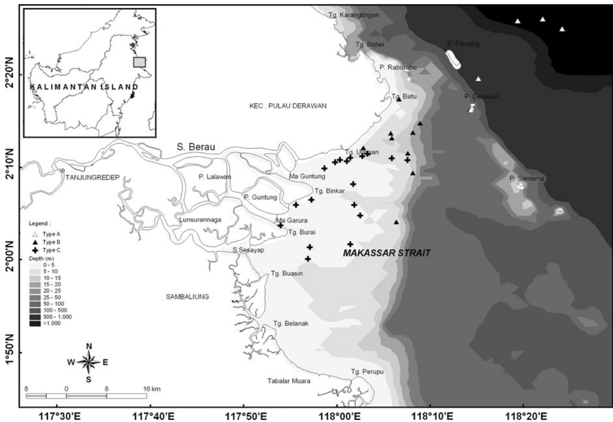
Fig. 1 The study area and field station locations in the Berau estuary, East Kalimantan Province, Indonesia ( source : Topographical Map). The stations are located in different types of waters as shown by the different symbols
