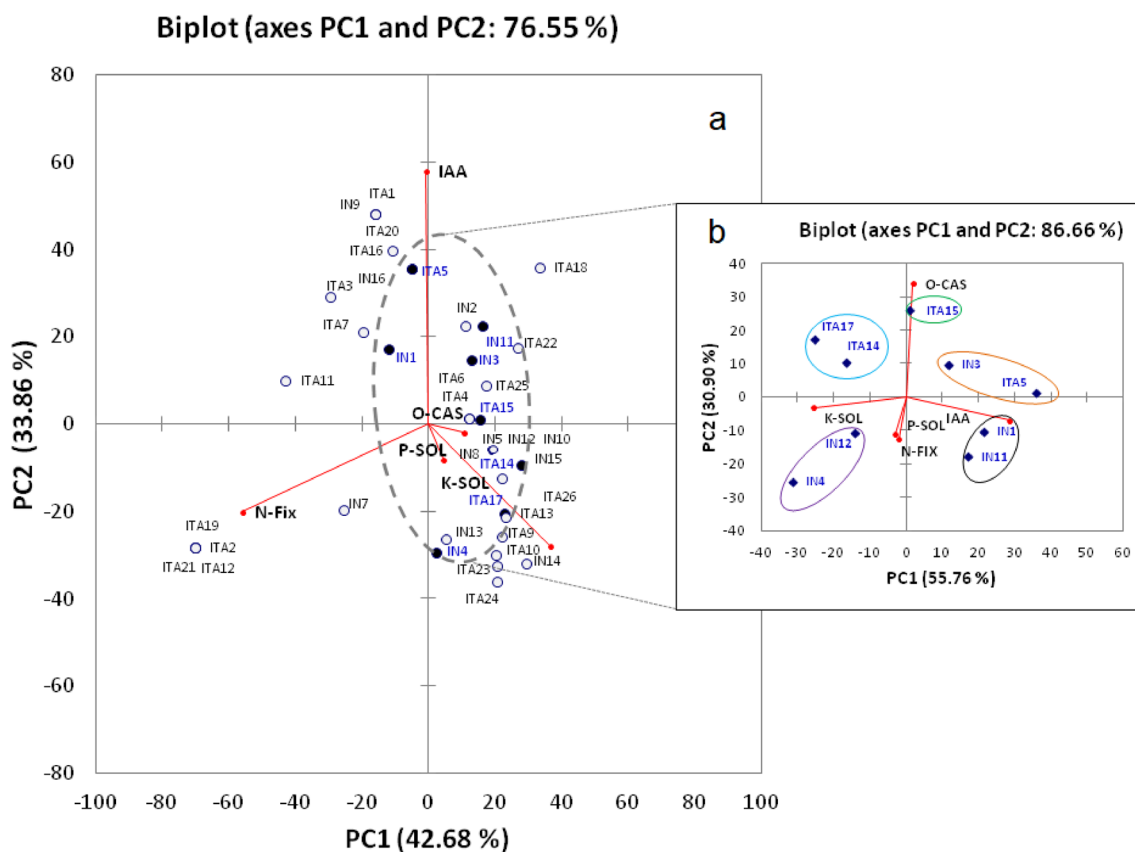
Fig. 3 a Biplot obtained by Principal Component Analysis (PCA) of all isolated strains, considering the first two components (PC1 42.68%, PC2 33.86%); b biplot of bacteria selected for the microbial
