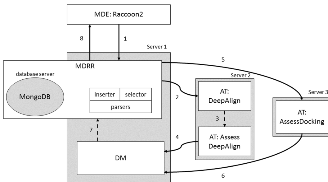
Fig. 9 Architecture of implementation of Scenario 1. Grey rectangles signify HTTP servers; white blocks signify elements. In this implementation, the MDRR contains a MongoDB database which
