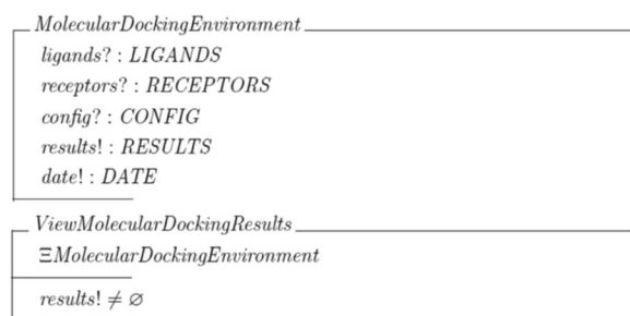
Fig. 4 Interface 1 described with Z notation using the input variables ligands? , receptors? , config? . Interfaces 2 and 3 described using the output variables results! and date! , with the condition that the results cannot be empty. LIGANDS defined as a set of LIGAND, RECEPTORS as a set of RECEPTOR, RESULTS as a set of RESULT. DATE defined as a set of characters describing a calendar date. Z symbols include \Xi to indicate no change of state
