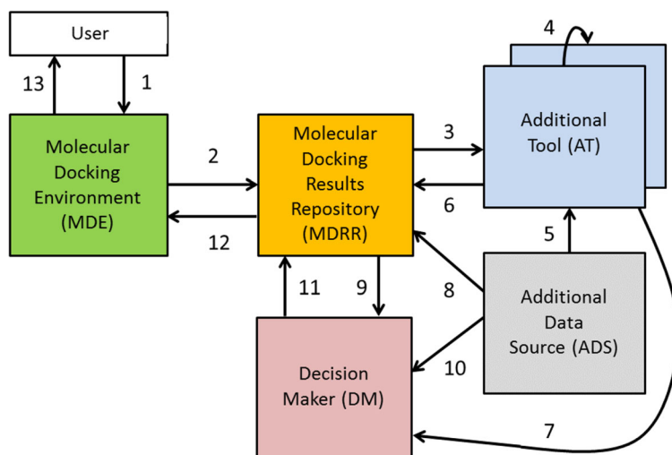
Fig. 1 Basic diagram of the framework - arrows show possible dataflow connections between element types. A user uploads input to the MDE (1) and docking data may be sent to the MDRR (2) which sends this or previous docking data to ATs (3). An AT may communicate with other ATs (4) or look up data in an ADS (5). An
