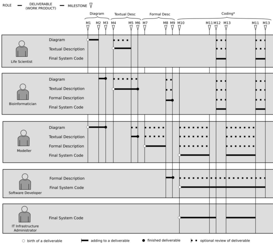
Fig. 5 Role-deliverable-milestone diagram of the proposed methodology. Roles on left, deliverables for each role in grey, milestones shown at top (M1: Diagram start; M2: Diagram ready for review; M3: Diagram ready; M4: Textual description start; M5: Textual description ready for review; M6: Textual description
