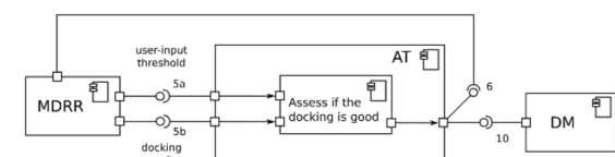
a The AT needed in Scenario 2 to assess docking results
