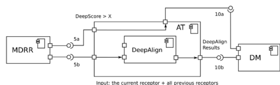
b The already implemented AT:DeepAlign for structural alignment
