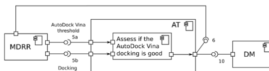
d The already implemented AT:AssessDocking for AutoDock Vina results
