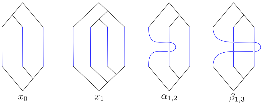
Fig. 4 Some generators of F_{br}
