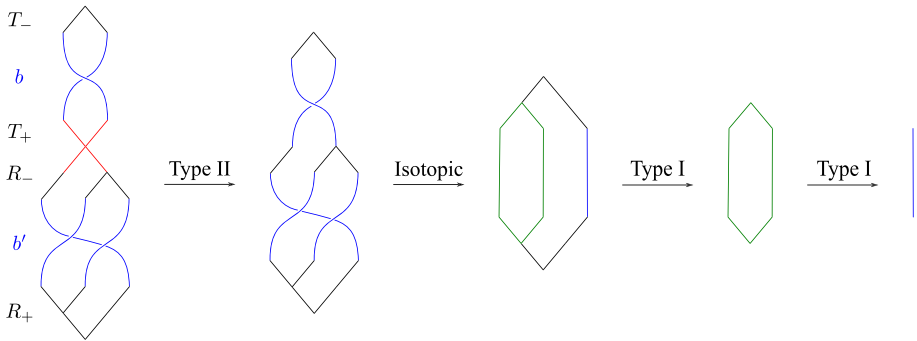
Fig. 3 Multiplication on V_{br}
