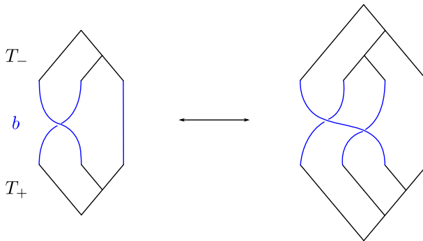
Fig. 1 A diagram (left) and an expansion of it (right)
