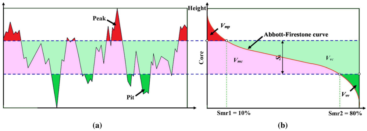
Fig. 11 Graphical presentation of the functional (volume) parameters: a an exemplary surface profile; b functional (volume) parameters of Abbott–Firestone curve according to ISO 25178. Adopted from (Macek 2021)
