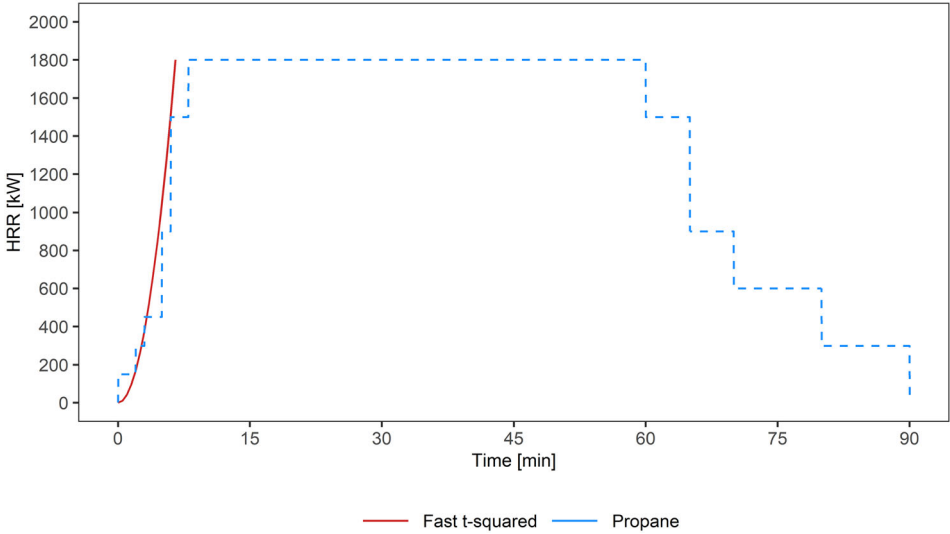
Figure 4. Propane HRR with time, alongside target fast t-squared growth rate.
