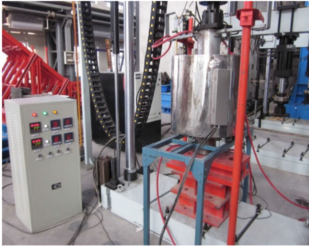
Figure 1. Electric heating furnace.
