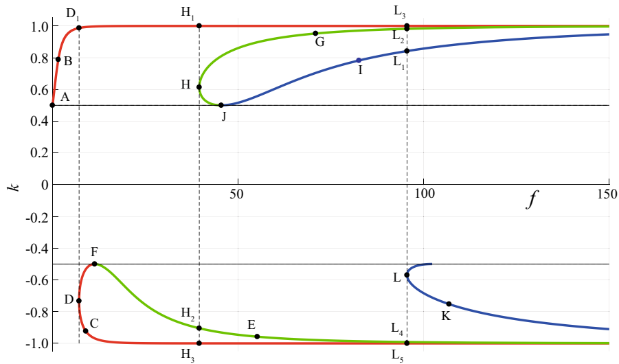
Fig. 6 A typical f - k plot for equilibrium configurations with 1 (red), 2 (green) and 3 (blue) inflection points for 0 < \alpha < \pi . (Color figure online)
