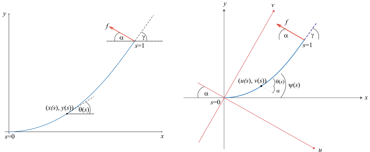
Fig. 1 The diagram on the left: the general configuration of the deformed rod with reference to the (x, y) coordinate frame under an end force f inclined at angle \alpha . The diagram on the right: the same deformed rod with reference to the (u, v) coordinate frame rotated clockwise through angle \alpha with respect to the (x, y) coordinate frame. In the (u, v) coordinate frame, the end force f acts along the u -axis. Note, \gamma = \theta(1) . (Color figure online)
