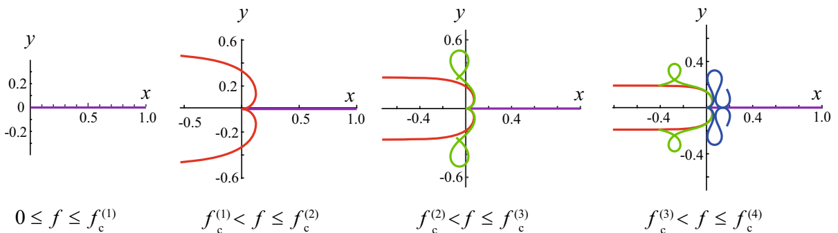
Fig. 5 The x - y shapes for equilibrium configuration with 1 (red), 2 (green) and 3 (blue) inflection points for \alpha = 0 and various values of f . The straight rod is represented by magenta. (Color figure online)
