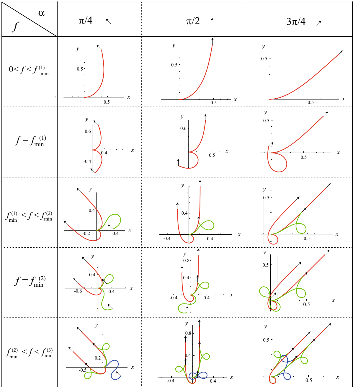
Fig. 3 The x - y shapes for equilibrium configuration with 1 (red), 2 (green) and 3 (blue) inflection points for \alpha = \pi/4, \pi/2 and 3\pi/4 and various values of f . (Color figure online)
