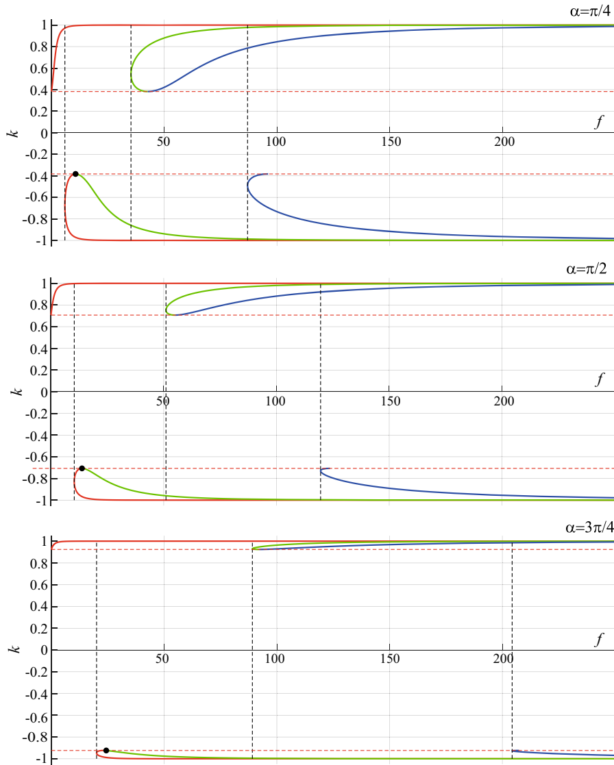
Fig. 2 f - k plots for equilibrium configurations with 1 (red), 2 (green) and 3 (blue) inflection points for \alpha = \pi/4, \pi/2 and 3\pi/4 . (Color figure online)
