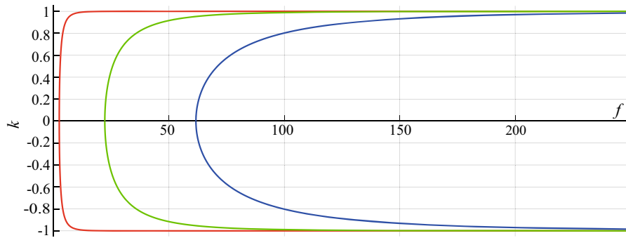
Fig. 4 f - k plots for equilibrium configurations with 1 (red), 2 (green) and 3 (blue) inflection points when \alpha = 0 . (Color figure online)
