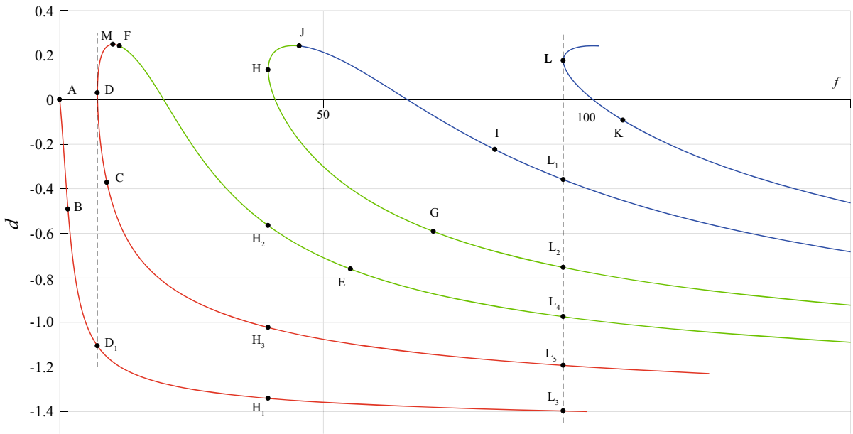
Fig. 8 A typical plot of d against f for equilibrium configurations with 1 (red), 2 (green) and 3 (blue) inflection points for 0 < \alpha < \pi . (Color figure online)
