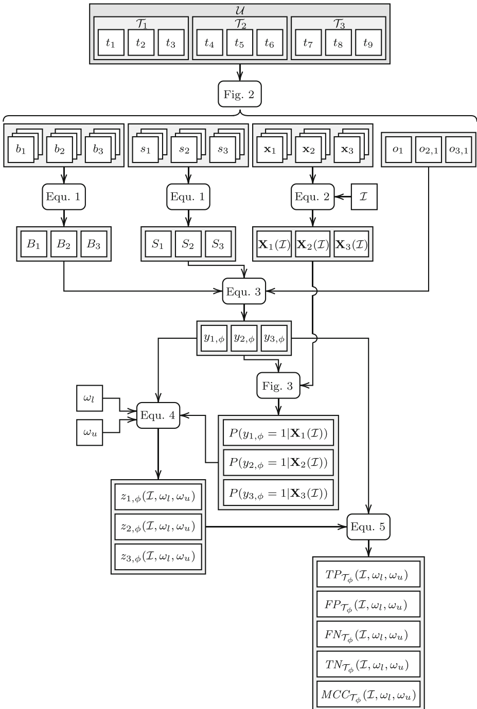
Fig. 4 An overview of how CANNIER-FRAMEWORK combines PYTEST-CANNIER and the general machine learning pipeline, with subject set \mathcal{U} , random sample \mathcal{I} , and thresholds \omega_l and \omega_u as input. It references previously defined figures and equations (e.g., Equ. 1 through 5 and Fig. 2 and 3)
