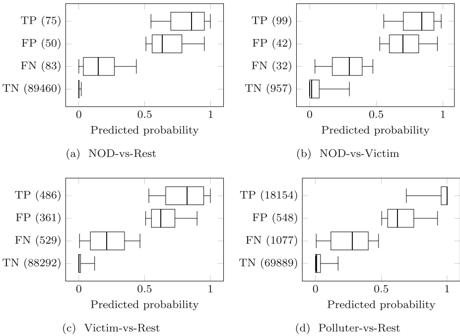
Fig. 10 The distribution of predicted probabilities for test cases in, and the frequencies of, each confusion matrix category, for each of the four flaky test classification problems. The data is based on the best pipelines from RQ1. Whiskers represent the range from the 5th to the 95th percentile and boxes represent the 25th to the 75th. Middle lines represent the median (50th)
