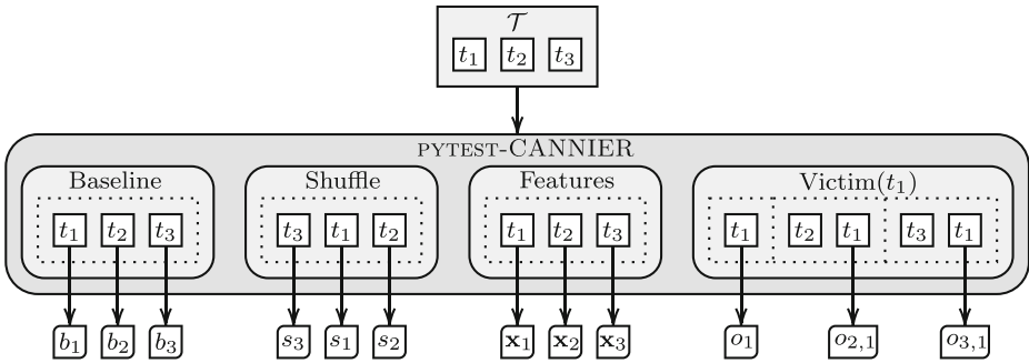
Fig. 2 As input, PYTEST-CANNIER takes a test suite \mathcal{T} = (t_1, t_2, t_3) and can be launched in four modes: Baseline , Shuffle , Features , or Victim . In the Baseline mode, the plugin runs the test suite in its original order and records the pass/fail outcome of every test case ( b_1, b_2, b_3 ). In the Shuffle mode, PYTEST-CANNIER executes the test suite in a random order and also records test case outcomes ( s_1, s_2, s_3 ). In the Features mode, the plugin produces a feature vector for each test case ( x_1, x_2, x_3 ). In the Victim mode, PYTEST-CANNIER takes a victim test case as an additional input ( t_1 ) and initially executes it in isolation to ascertain its expected outcome ( o_1 ). Then, the plugin executes every other test case in a separate process with the victim immediately following and records its outcome ( o_{2,1}, o_{3,1} ). This is to identify polluters of the victim
