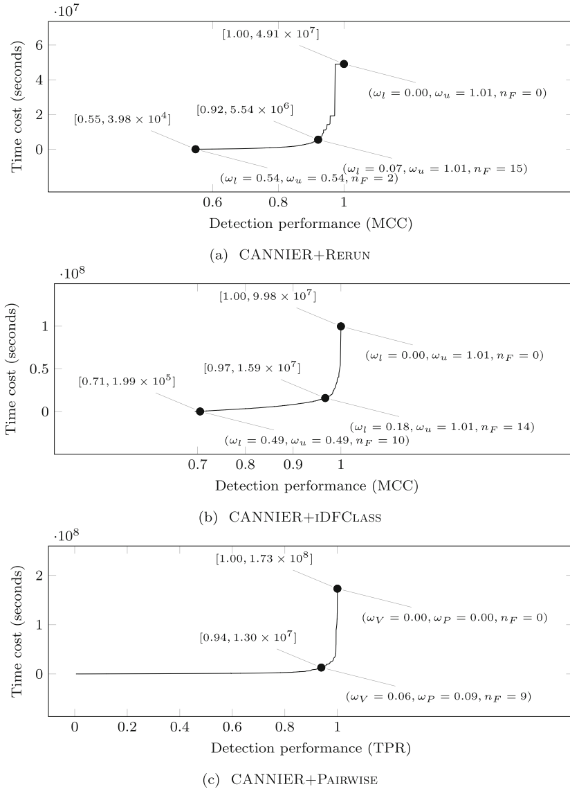
Fig. 8 The Pareto fronts of detection performance and time cost for the application of CANNIER to the three rerunning-based detection techniques. From right-to-left, the first pin on each curve is at the point representing the original rerunning-based technique. The second is at the point representing the balanced application of CANNIER. For CANNIER+RERUN (a) and CANNIER+iDFCLASS (b), the third is at the point representing pure machine learning-based detection. There is no third pin for CANNIER+PAIRWISE (c) because it is not possible to use a pure machine learning-based approach in this context (see Section 5.2.4). Above each pin in square brackets is the detection performance and time cost with respect to the whole subject set. Below in parentheses are the parameters
