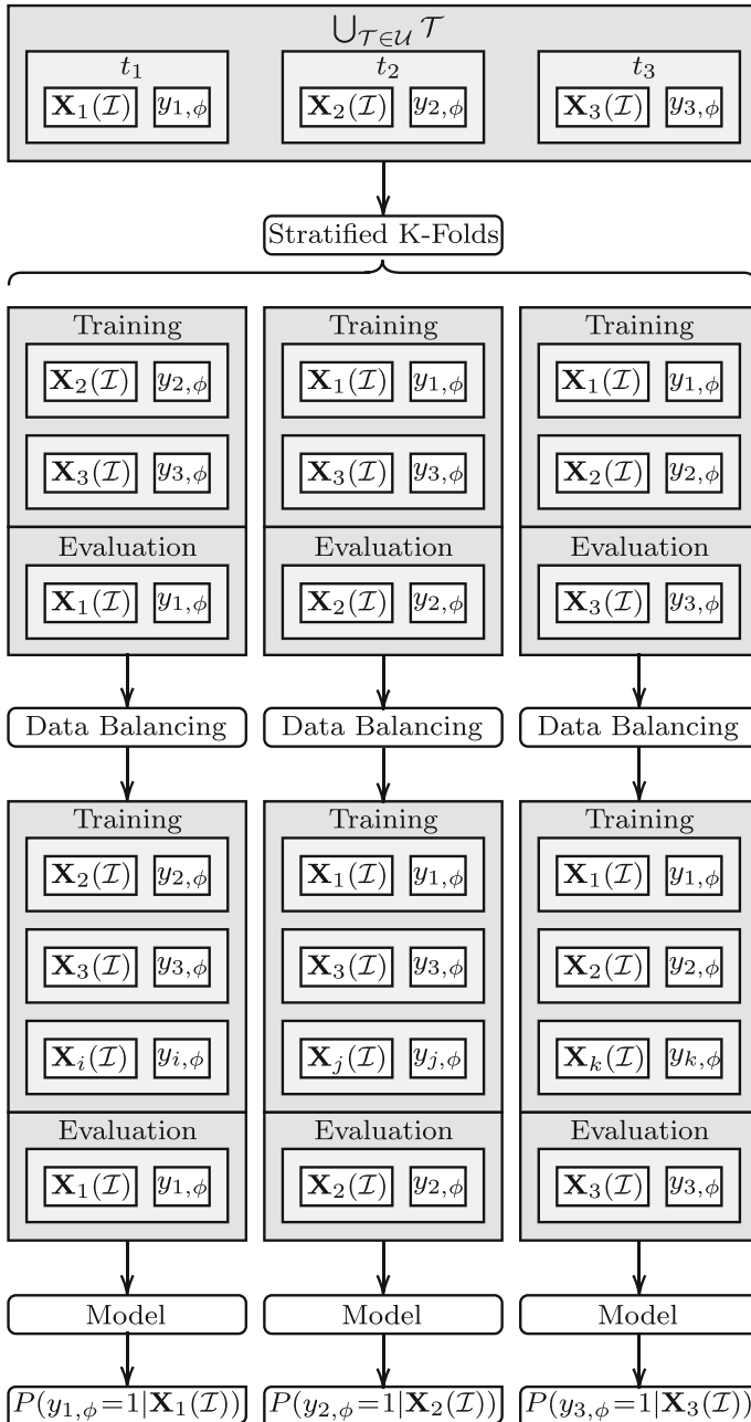
Fig. 3 CANNIER-FRAMEWORK performs stratified k-folds cross validation upon the set of all test cases in the subject set, \cup_{\mathcal{T} \in \mathcal{U}} \mathcal{T} . Following this, it applies a data balancing technique to the training portion of each fold. The framework then trains a machine learning model using the mean feature vectors \mathbf{X}_i(\mathcal{I}) , and ground-truth labels y_{i,\phi} , of every test case t in each training portion. Finally, for each fold, CANNIER-FRAMEWORK applies the trained model to the feature vectors of every test case in the evaluation portion. Since the evaluation portion of each fold is unique, every test case ends up with a predicted probability of being in the positive class, P(y_{i,\phi} = 1 | \mathbf{X}_i(\mathcal{I}))
