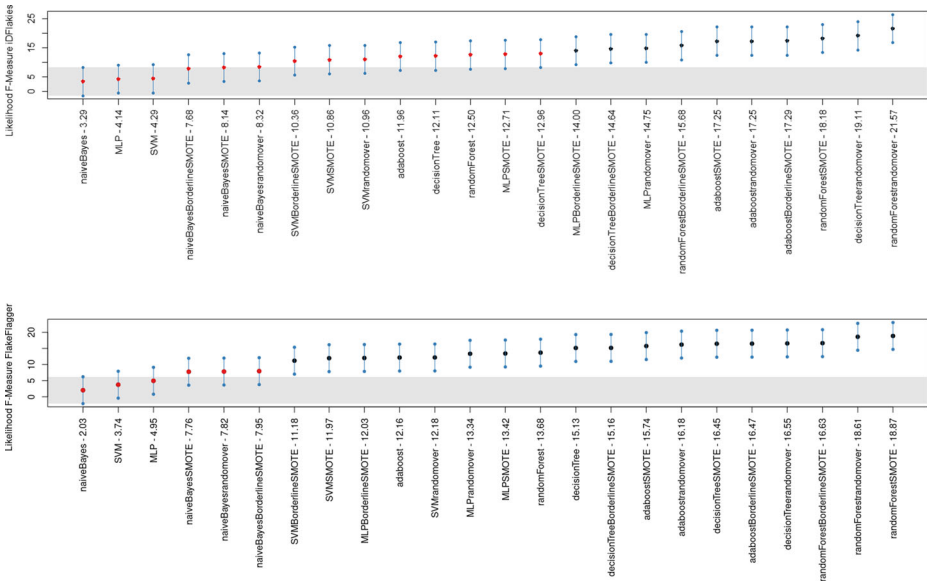
Fig. 3 The likelihood of each technique in within prediction in Nemenyi rank in terms of F-Measure. Circle dots are the median likelihood, while the error bars indicate the 95% confidence interval. 60% of likelihood means that a classification technique appears at the top-rank for 60% of the studied projects
