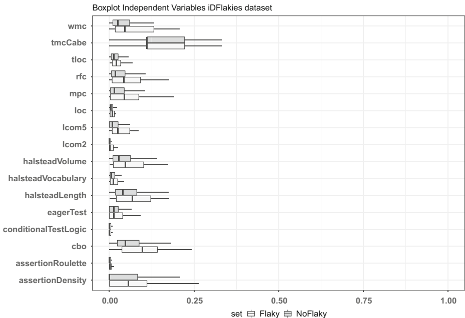
Fig. 1 RQ 1 . Analysis of the metric profiles of flaky and non-flaky tests on the IDFLAKIES dataset
