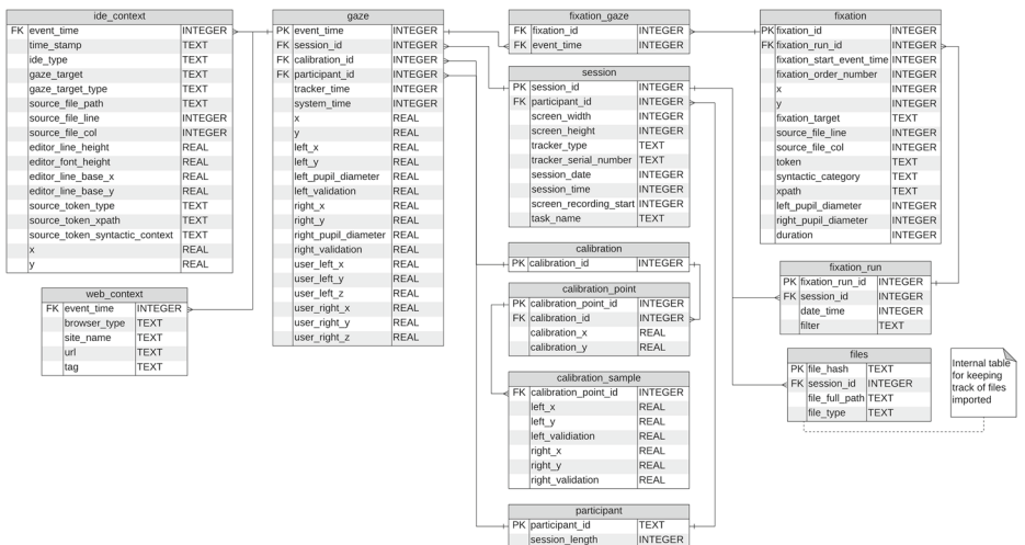
Fig. 4 An overview of the iTrace Toolkit Relational Database Schema
