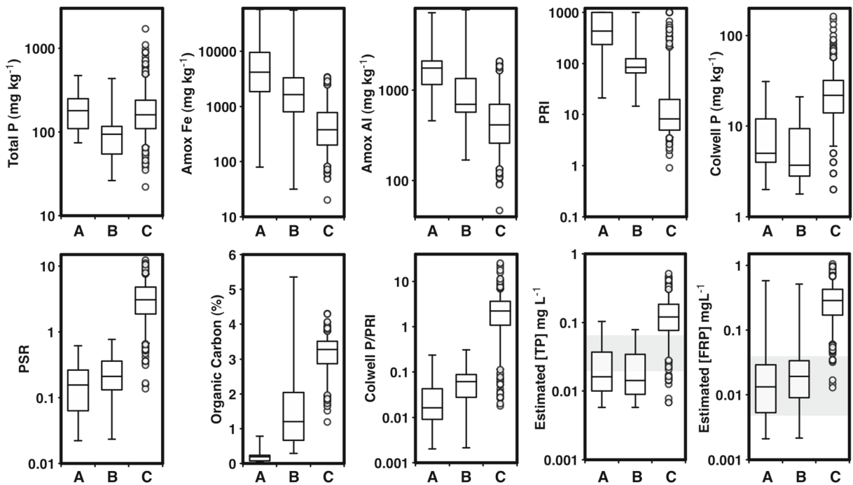
Fig. 6 Box and whisker plots comparing chemical characteristics of (A) <75- \mu\text{m} fraction of stream bank soil, (B) whole stream bank soil and (C) <2-mm fraction of catchment soils. Whiskers show 5th
