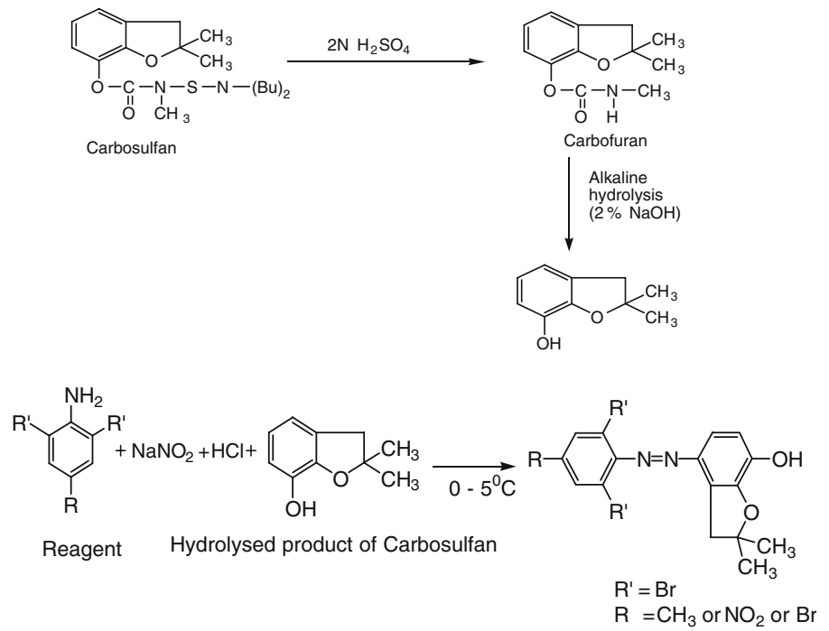
Fig. 2 Interactions of carbosulfan with coupling reagents
