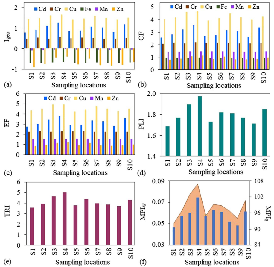
Fig. 3 Evaluation of sediment contamination using a I_{geo} , b CF, c EF, d PLI, e TRI, and f MPI
