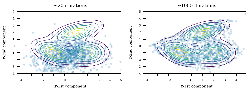
(b) Mixture of three 2D Gaussians. The contour lines indicate the target distribution, and the scattered points correspond to generated values.
