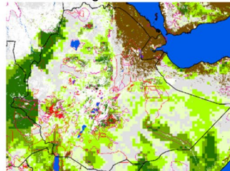
p climate change with 2015 land cover
