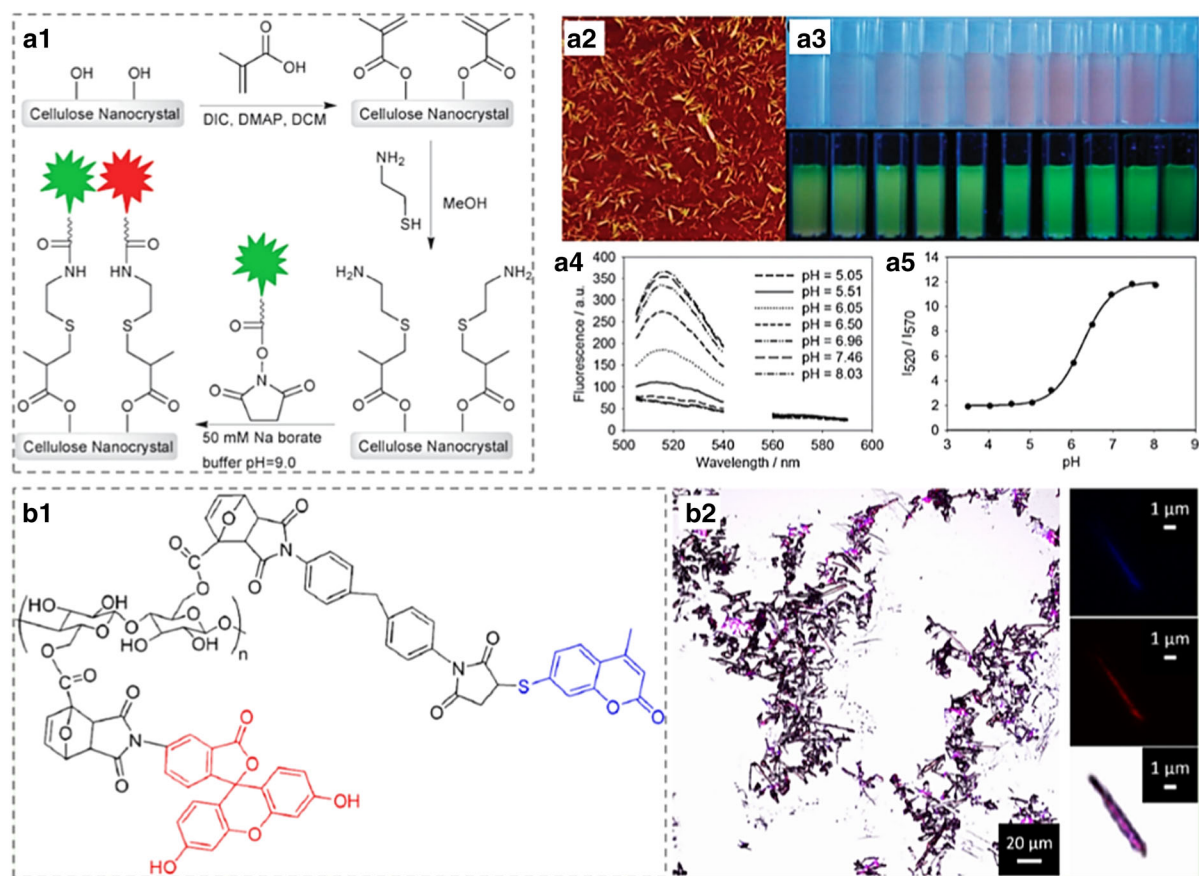
Fig. 10 a Dual fluorescent labelled CNCs for pH sensing. (a1) Synthesis of fluorescent labeled CNCs with succinimidyl ester dyes; (a2) AFM image of fluorescent labeled CNCs; (a3) suspensions of pH responsive fluorescent labeled CNCs (0.1 wt%) at increasing pH values; (a4) emission spectra of pH responsive fluorescent labeled CNCs at different pH values ( \lambda_{\text{ex}} = 490 and 540 nm for FITC and RBITC, respectively); (a5) plot of intensity ratios versus pH values. Reprinted from Nielsen
