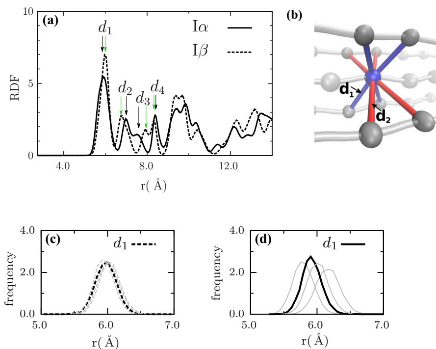
Fig. 2 a shows RDF for the C4 atoms in the crystalline cellulose I\alpha (solid line) and I\beta (dashed line). The positions of the first four peaks along the r -axis are indicated by the vertical arrows next to the symbol “ d_i ” where the subscript i ranges between 1 and 4. It counts the peaks in the ascending order. The green arrows correspond to I\beta and those in the black color to I\alpha . b shows four cellulose chains surrounding one central chain in the C4 representation. The eight C4 atoms which are closest to an arbitrary C4 atom (in blue) from the central chain are
