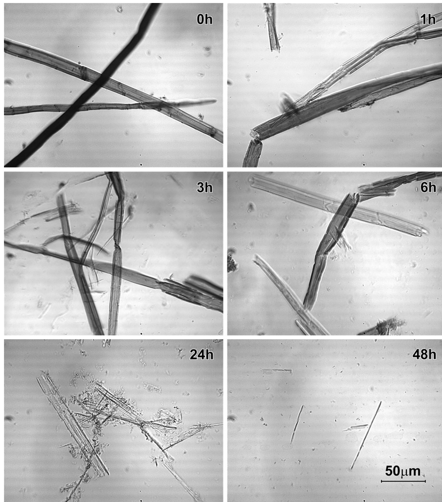
Fig. 2 Microscopic images at \times 200 magnification showing the gradual degradation of poplar cellulosic pulp fibers during 48 h hydrolysis mediated by the preparation NS-22086 (50 °C, pH 5.0)
