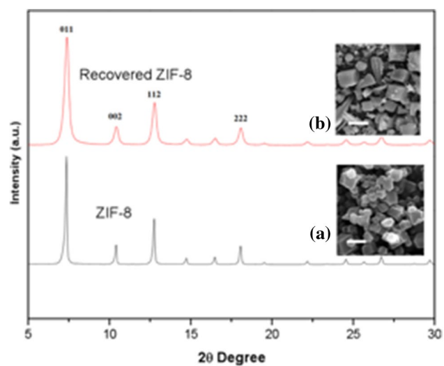
Fig. 7 Powder X-ray diffraction patterns of ZIF-8 (before use) and recovered ZIF-8 (after 3rd cycle). a SEM pictures of ZIF-8 (scale bar: 2 \mu\text{m} ), b SEM micrographs of recovered ZIF-8 (1 \mu\text{m} )
