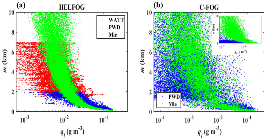
Fig. 10 Variation of visibility (MOR) with LWC ( q_l ) from (a) HELFOG, and (b) C-FOG fog events. Results from the C6 event are shown in the inset. The blue dots are from the PWD sensors, red from WATT (HELFOG only) and all green dots are results from the Mie calculation. Data shown here are 1-min averages
