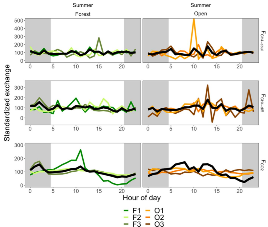
Fig. 5 Hourly standardized fluxes of forest and open ponds during summer of F_{CH_4\text{-ebul}} , F_{CH_4\text{-diff}} and F_{CO_2} . Black lines indicate the overall mean. Grey area indicates night hours
