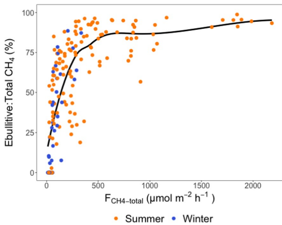
Fig. 4 Average F_{CH_4\text{-total}} plotted against average F_{CH_4\text{-ebul}} : F_{CH_4\text{-total}} for each individual day for all ponds during summer and winter. Black line is fitted with a local polynomial regression model
