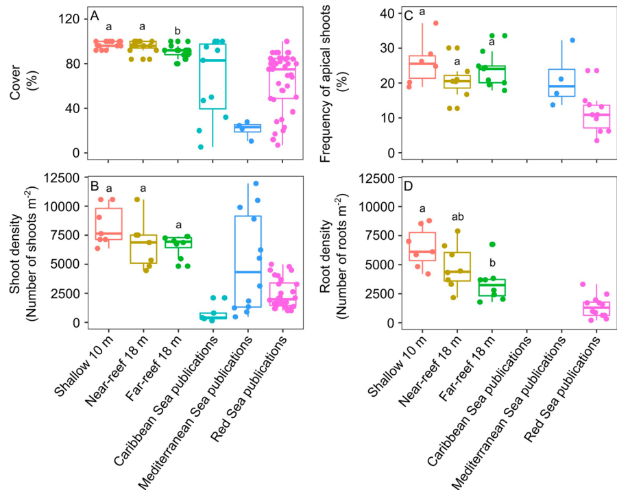
Fig. 2 Meadow characteristics in Oranjestad Bay and comparisons with previous studies. A Percent cover, B shoot density, C frequency of apical shoots, and D root density. Different small letters indicate statistical significant differences between study sites (Tukey HSD post hoc test, p < 0.05 ). No statistical analysis was done for the data collected from previous studies. The three left boxplots represent measured data while the three right boxplots represent published data. Boxplots represent the medians and quartiles (0.25, 0.75)
